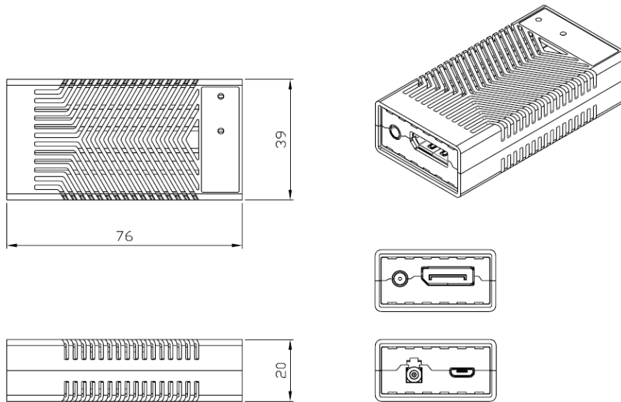
Dimensions (L*W*H): 39 x 76 x 20 mm
